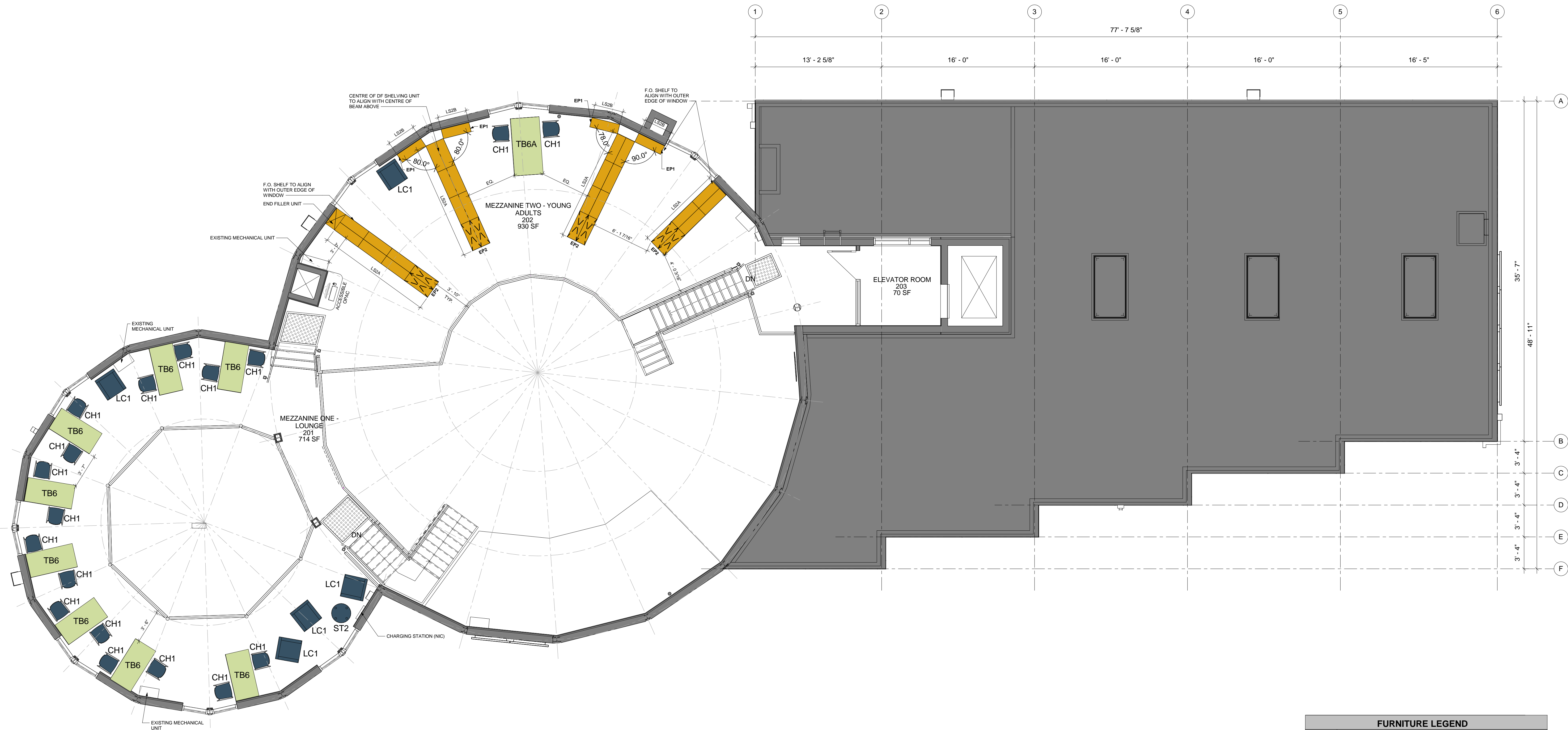
1 FURNITURE PLAN - MEZZANINE 3/16" = 1'-0"
